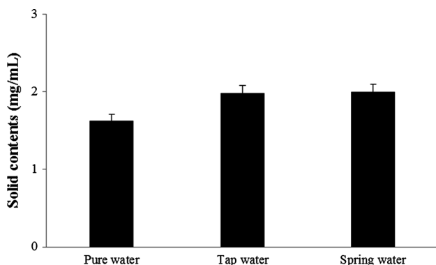
Fig. 3 Effect of water quality on the solid content in Fuding white tea infusions
