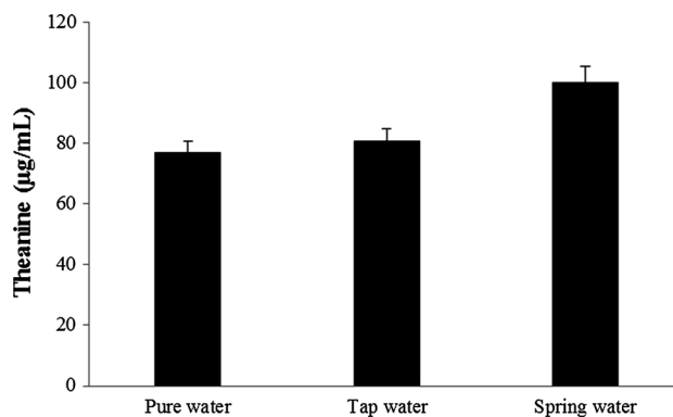
Fig. 4 Effect of water quality on the theanine content in Fuding white tea infusions
